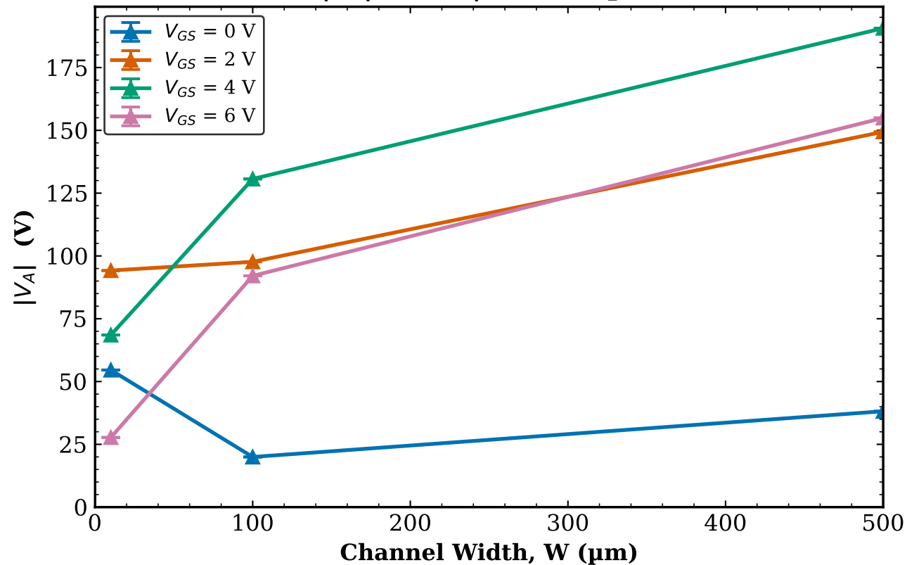
TFT1 Transistor 1 |V_A| vs W | L = 20\text{ }\mu\text{m}
